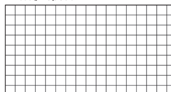
2-Way repeat
